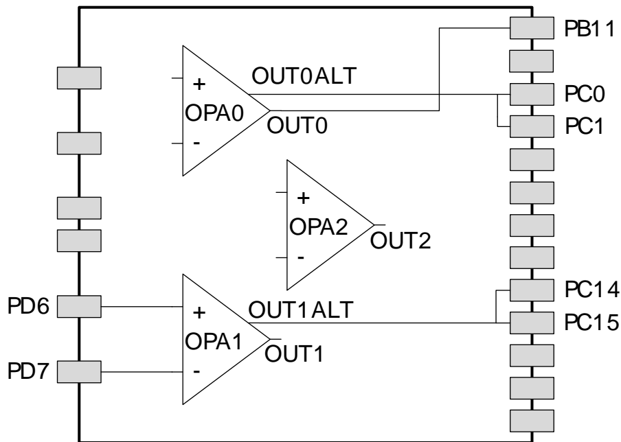
Figure 4.2. Opamp Pinout
